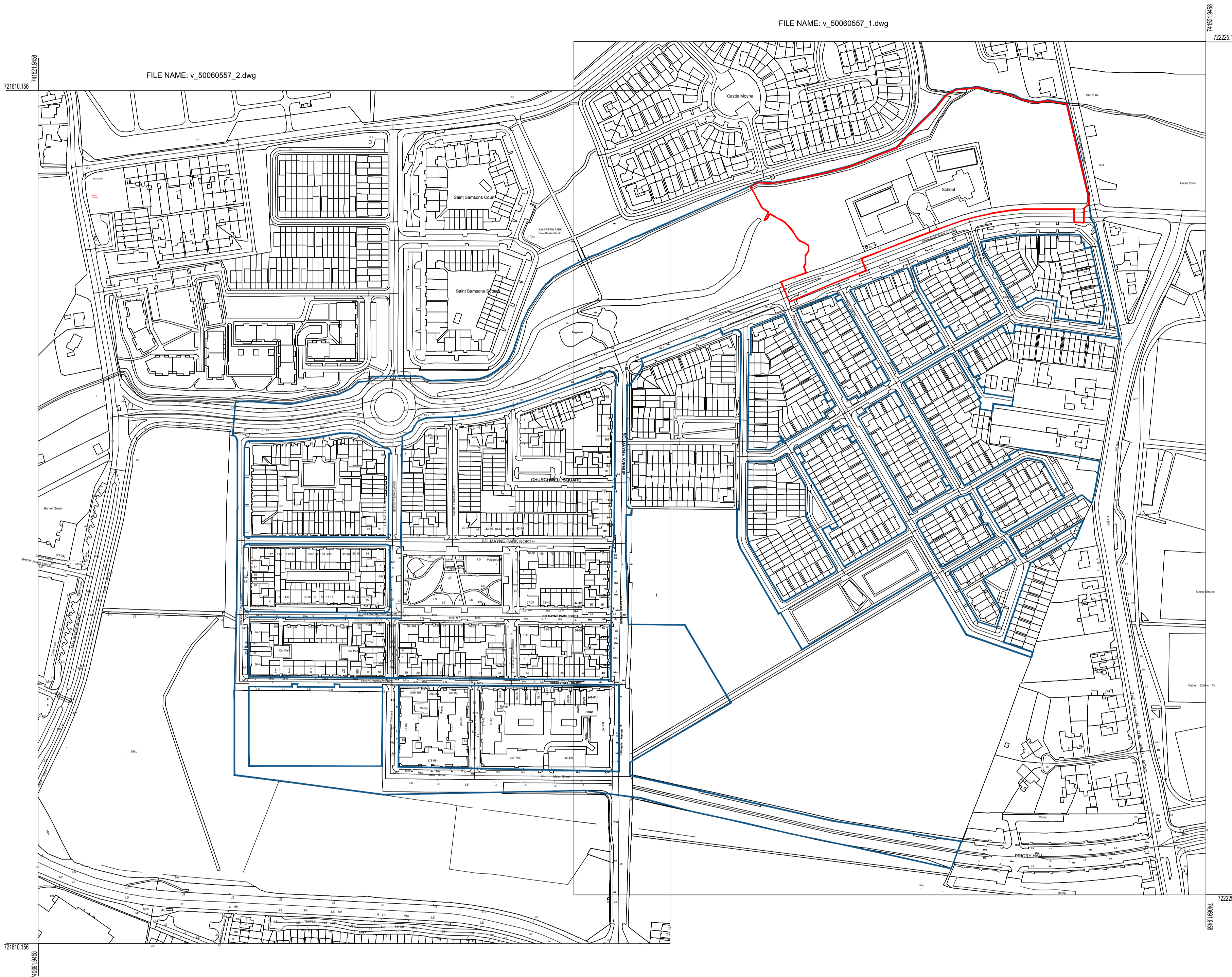
SITE LOCATION PLAN - LANDS IN APPLICANT'S OWNERSHIP SCALE 1:2500
